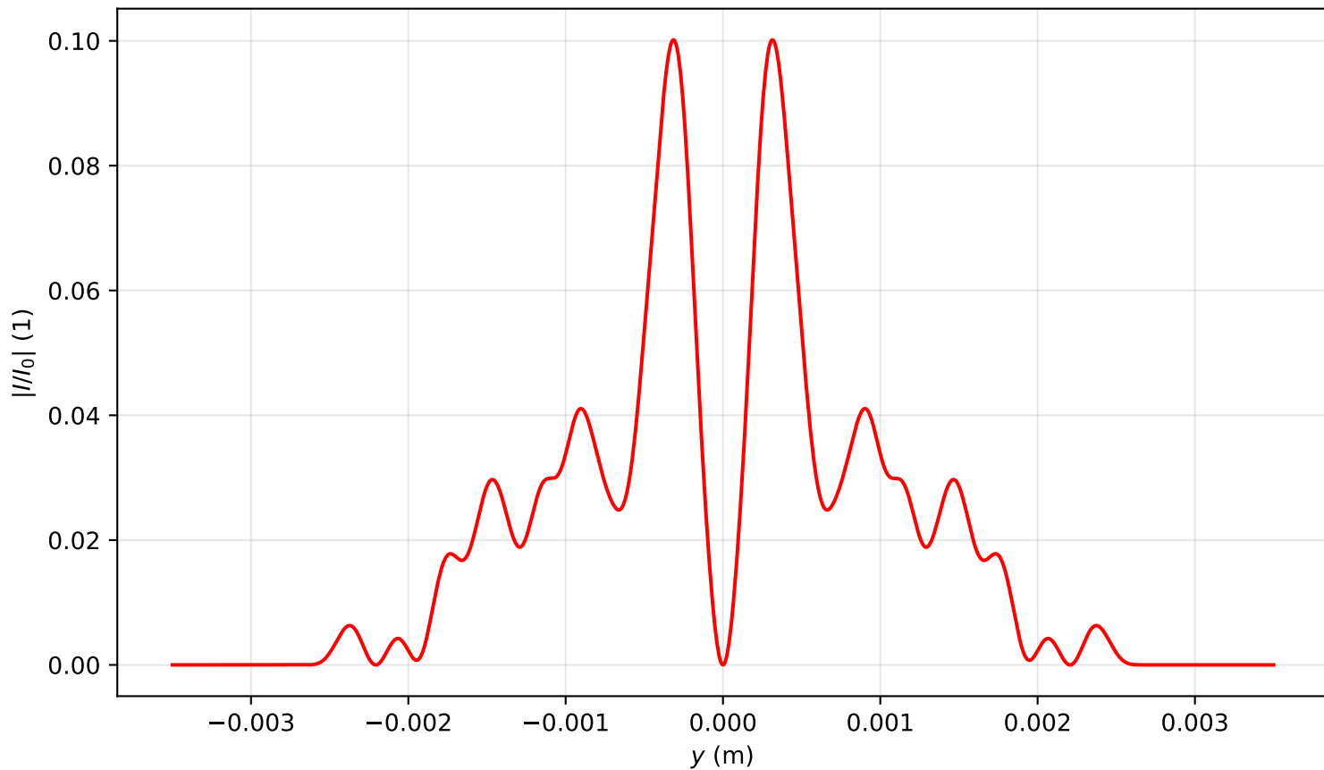
Intensity profile I(x=0, y, z=2.468)/I_0 , P_{in}=8.0P_{cr} , artificial time
